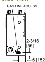
SL-950TR Side View
